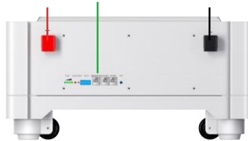
Installation Diagrams of 5KWH
