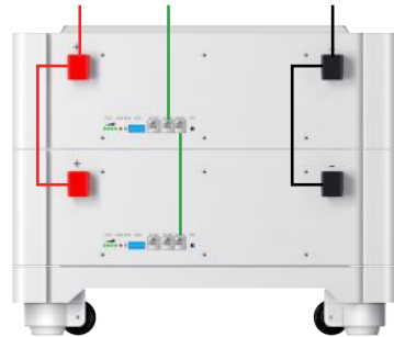
Installation Diagrams of 10KWH
